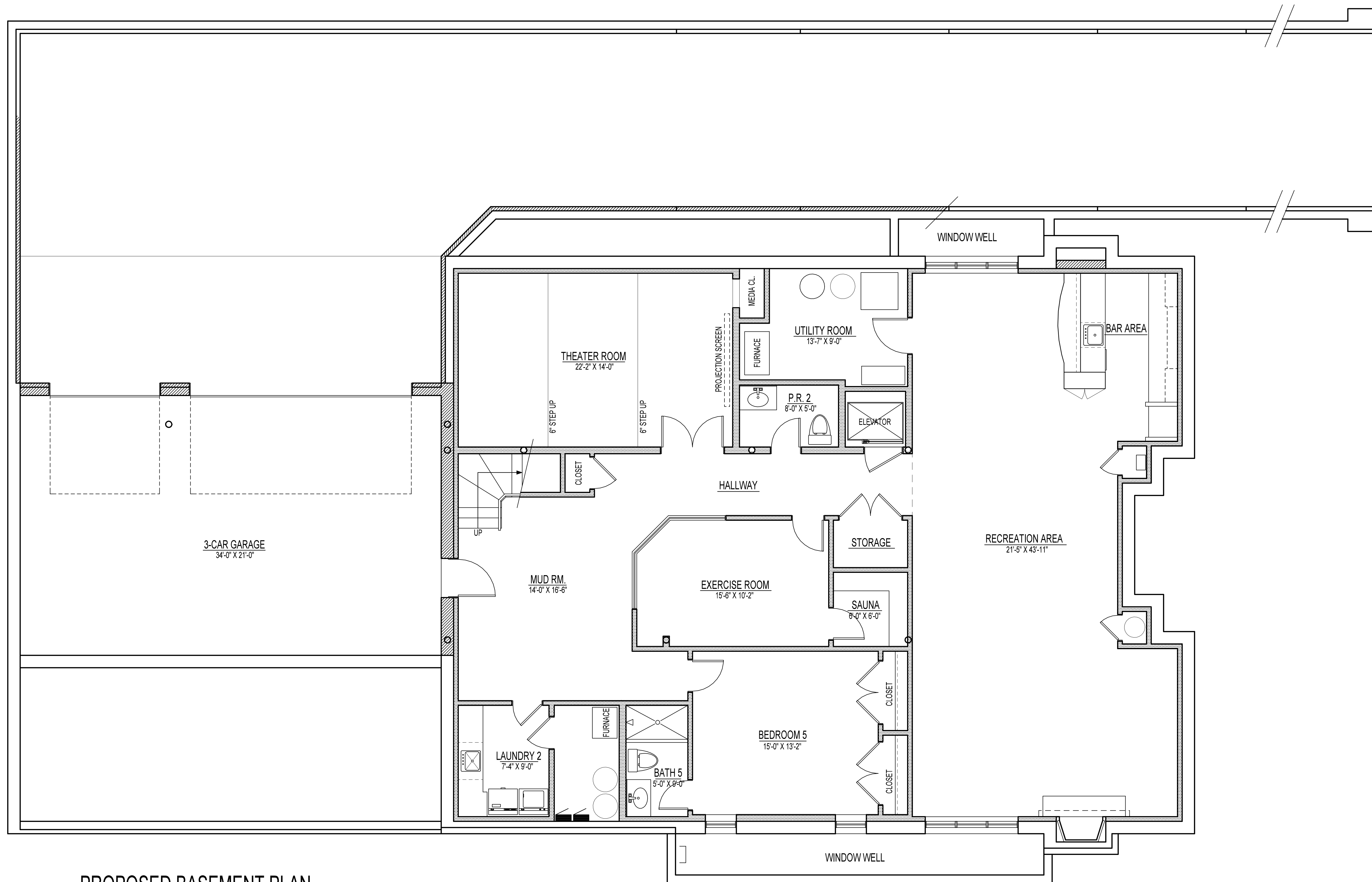
PROPOSED BASEMENT PLAN
