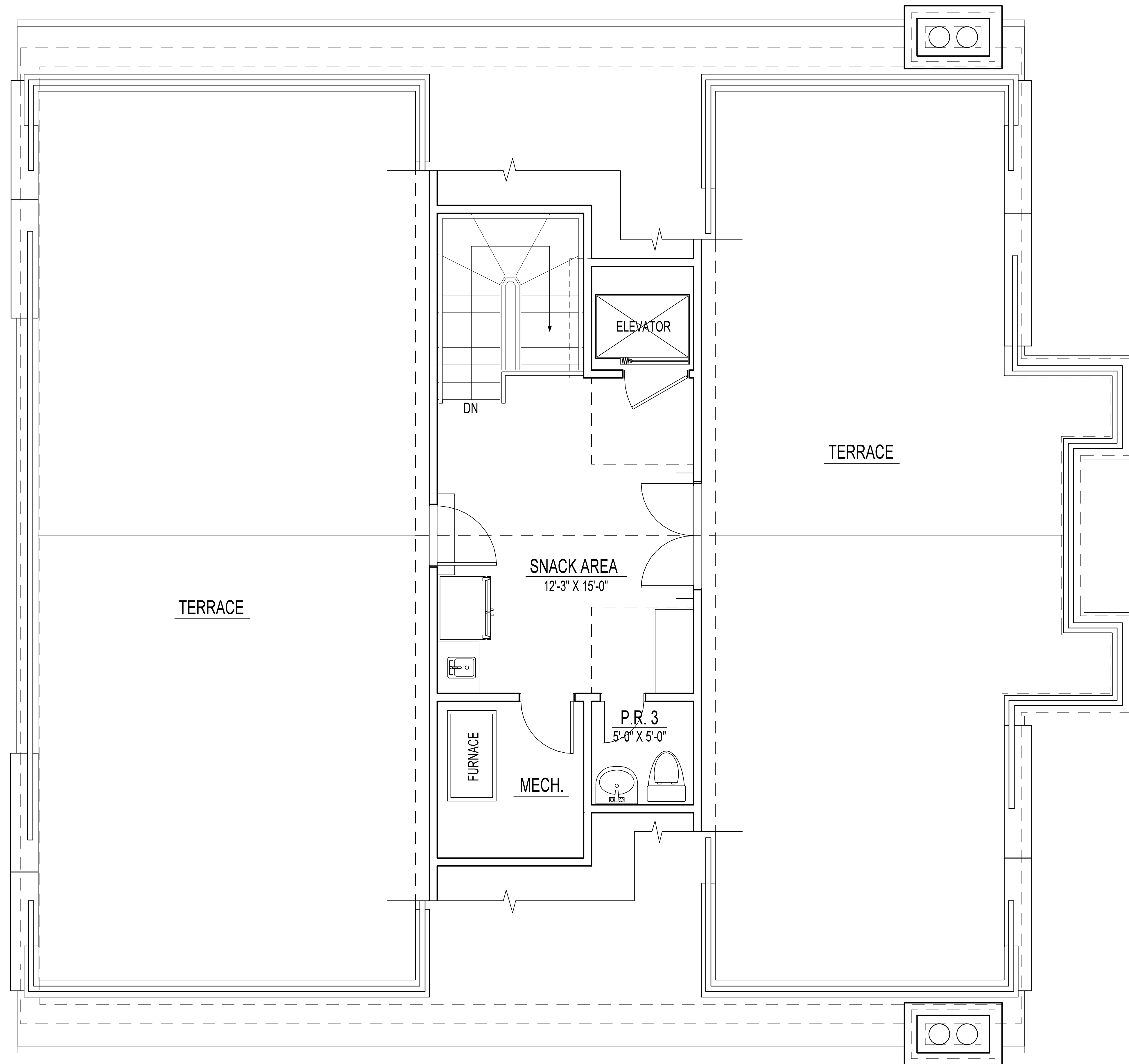
PROPOSED 3RD FLOOR PLAN
