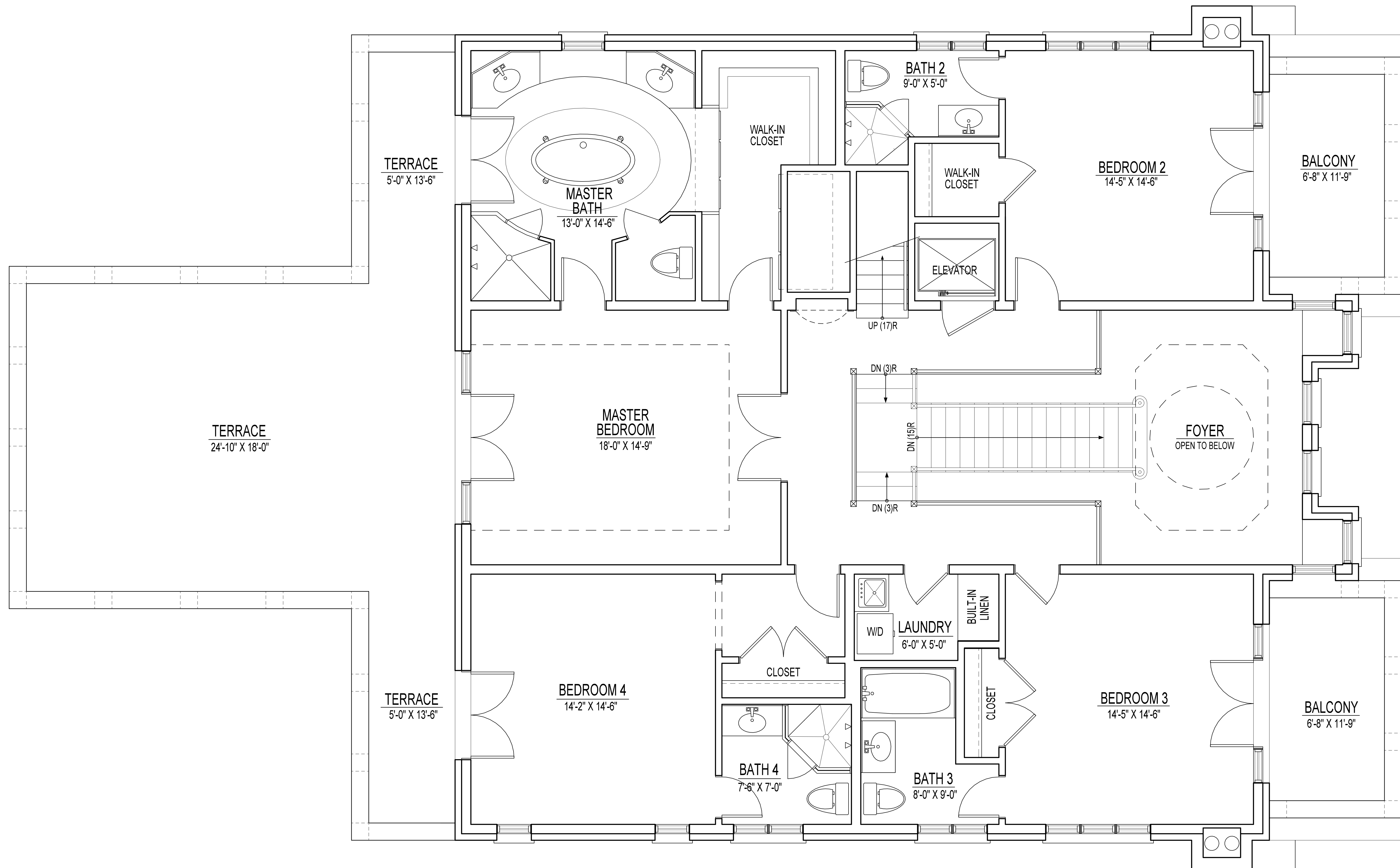
PROPOSED 2ND FLOOR PLAN
